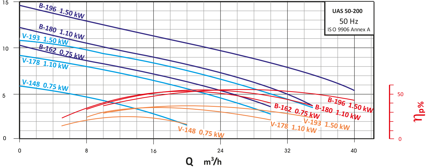
Performans Eğrisi / Performance Curves
