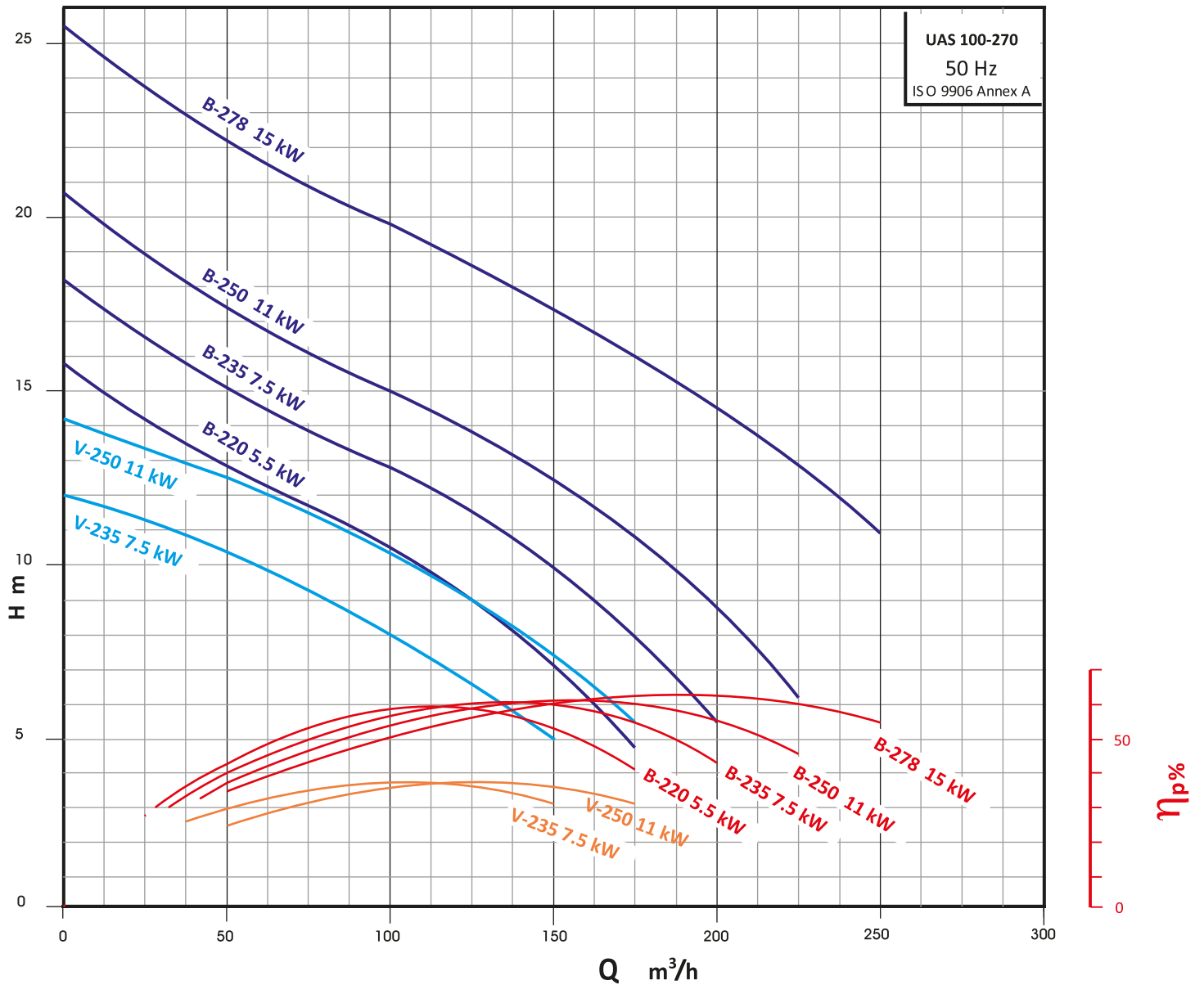
Performans Eğrisi / Performance Curves
