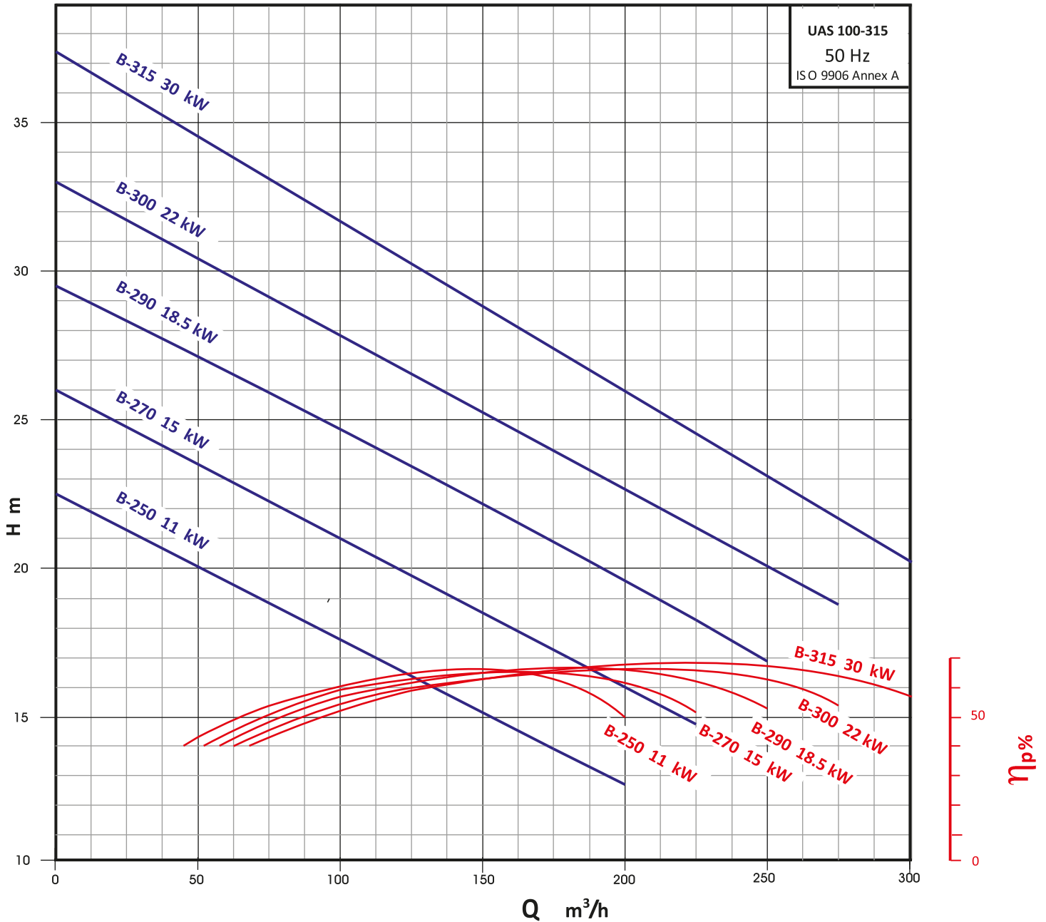
Performans Eğrisi / Performance Curves
