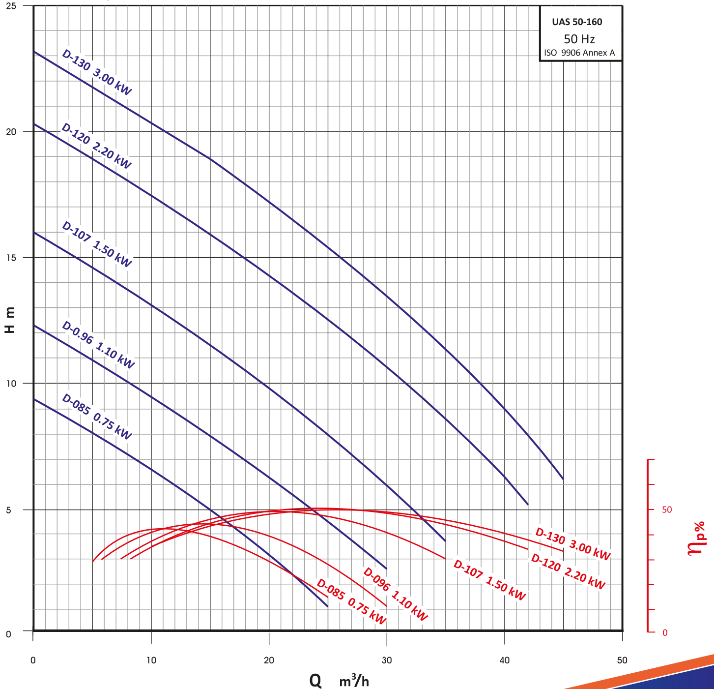
Performans Eğrisi / Performance Curves
