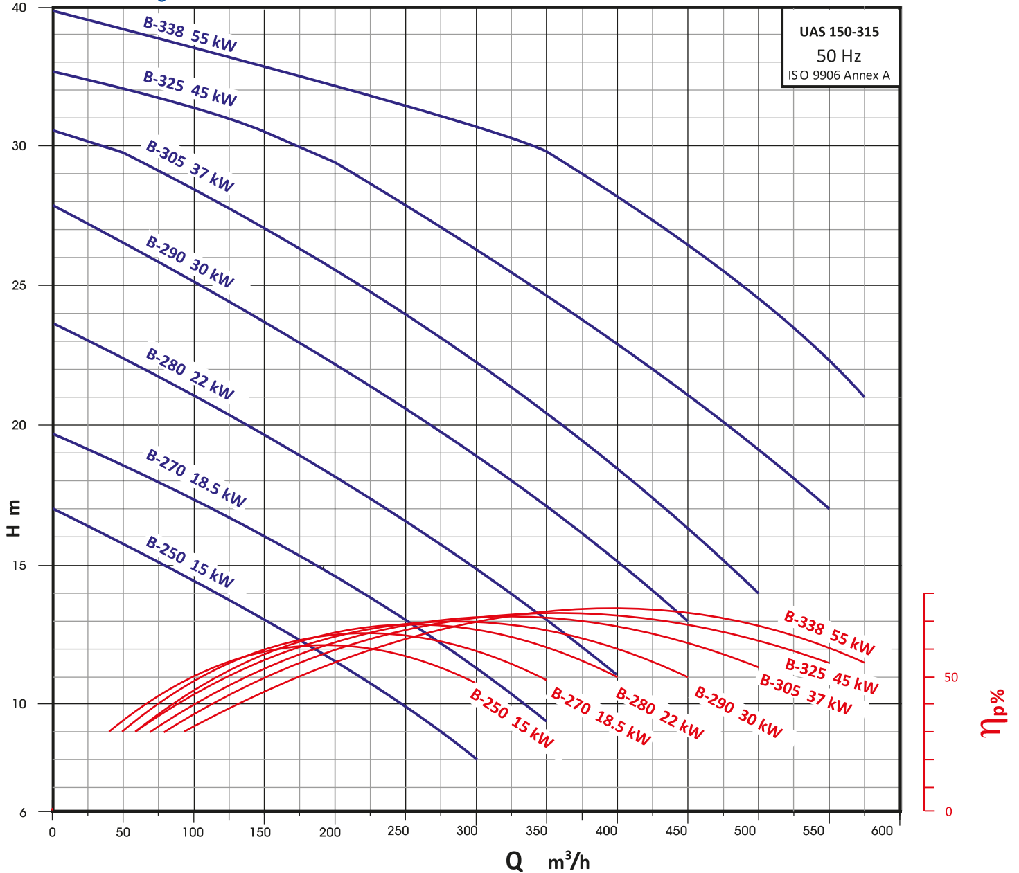
Performans Eğrisi / Performance Curves
