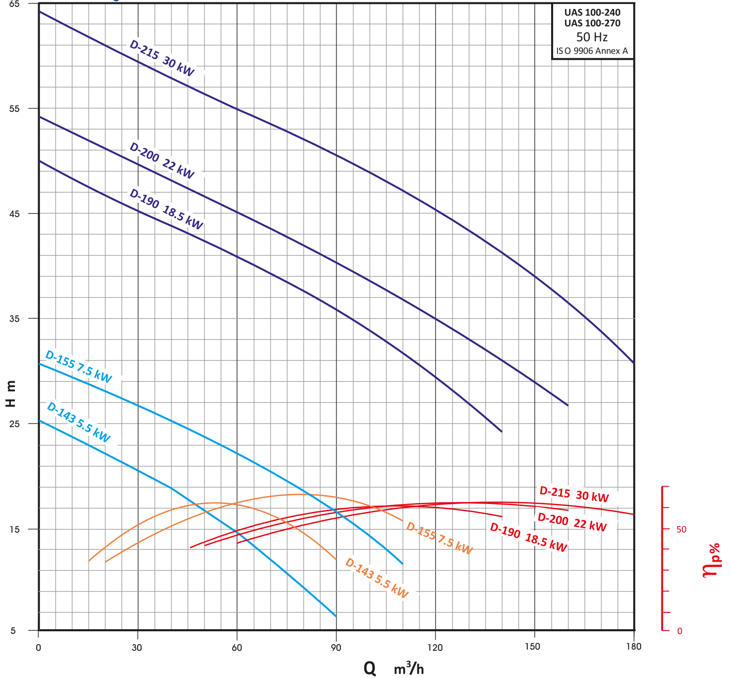
Performans Eğrisi / Performance Curves
