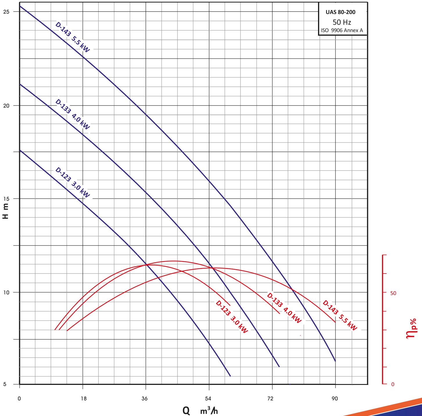
Performans Eğrisi / Performance Curves
